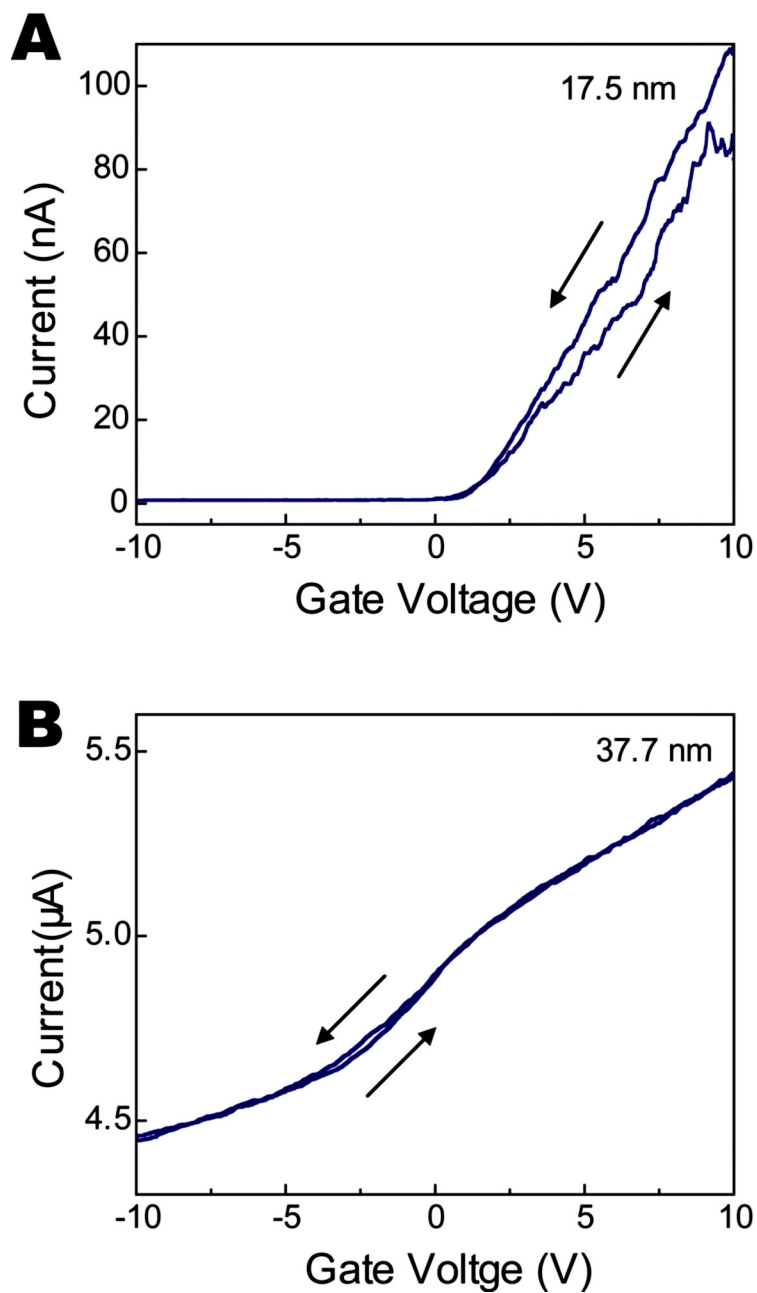
Fig. S1. Representative examples of I-V_g curves measured for both sweep directions for small (A) and large (B) diameter NWs after 1 cycle of oxidation and etching, respectively. Diameters labeled in this figure are as-grown diameters.
